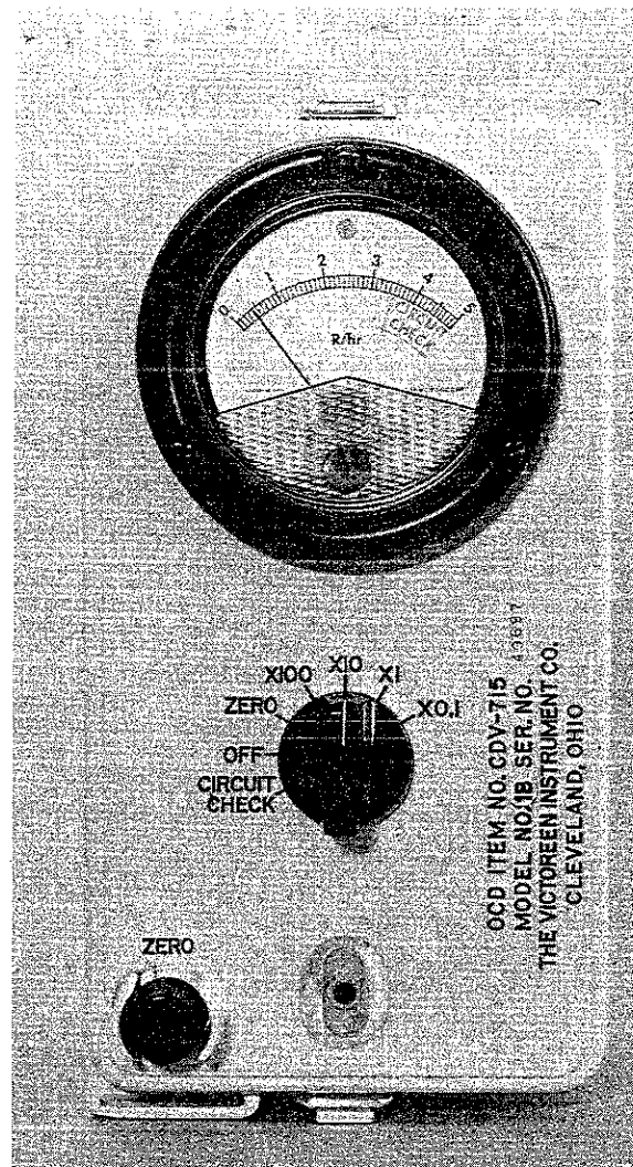
Figure 3-3. The survey meter dial reading is 0.4. This reading is multiplied by 10 to get the radiation exposure rate reading because the range-selector switch points to "X10." The radiation exposure rate is 4 R/hr.
