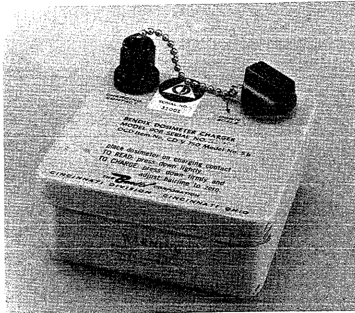
Figure 2-3. Dosimeter charger.
