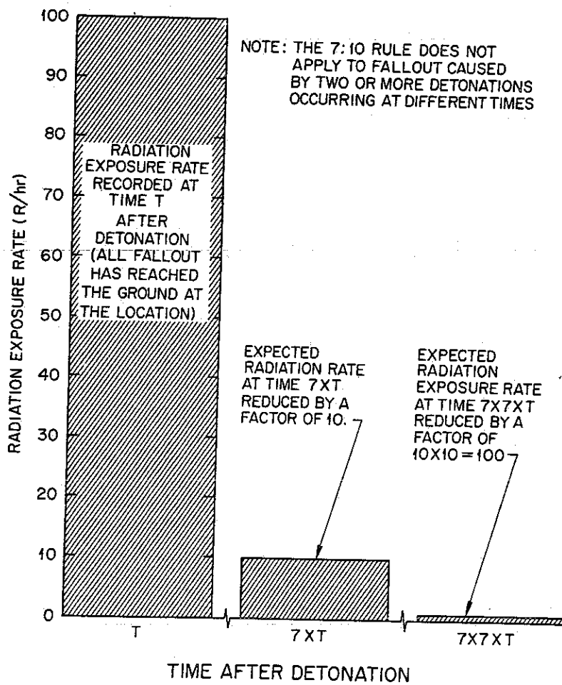
Figure 1-2. Illustration of the seven-ten rule. The time "T" after detonation is the age of the fallout.
