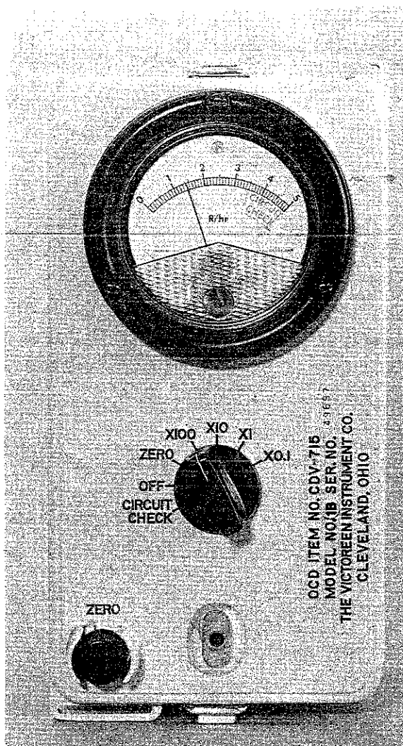
Figure 3-2. The survey meter dial reading is 1.4. This reading is multiplied by 100 to get the radiation exposure rate reading because the range-selector switch points to "X100." The radiation exposure rate is 140 R/hr.
