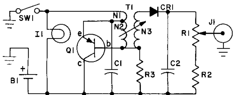
Figure 2 — Schematic
